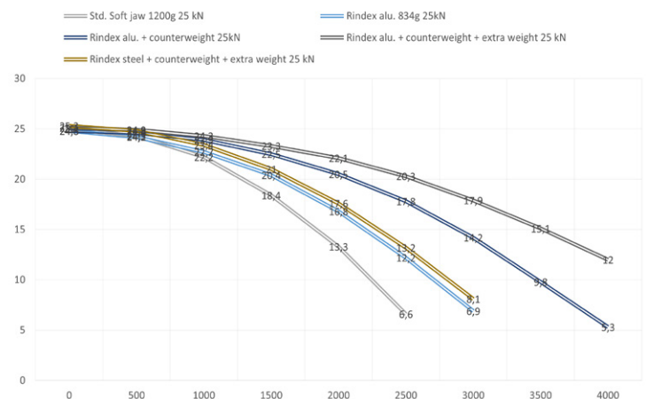
JAWS AND COUNTERWEIGHTS AT DIFFERENT CLAMPING FORCE (kN) AND SPINDEL SPEED (RPM)
